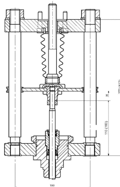
Attachement yoke
