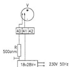
Execution: with resistance transmitter with capacity position transmitter
