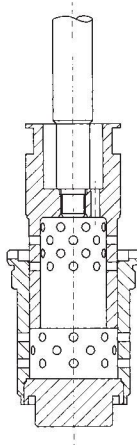
Two-step pressure reduction
